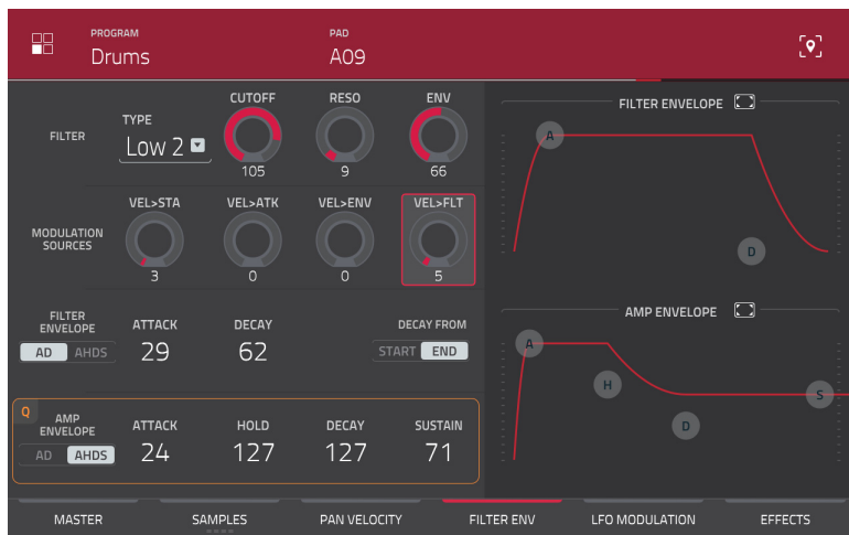
The Filter Envelope tab of a drum program.
