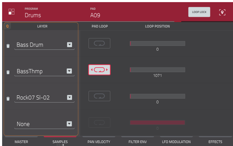
The fourth Samples tab for a drum program.
